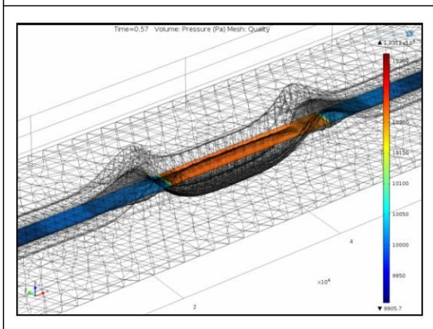
Figure 6: Pressure Profile in the Channel (Top) and Fluid Flow Rate (Top) at the Right Throttle at 0.57 s Time
