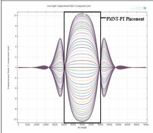
Figure 5: Deformations of a Membrane in a Central Longitudinal Cross-Section for Different Applied Voltages
