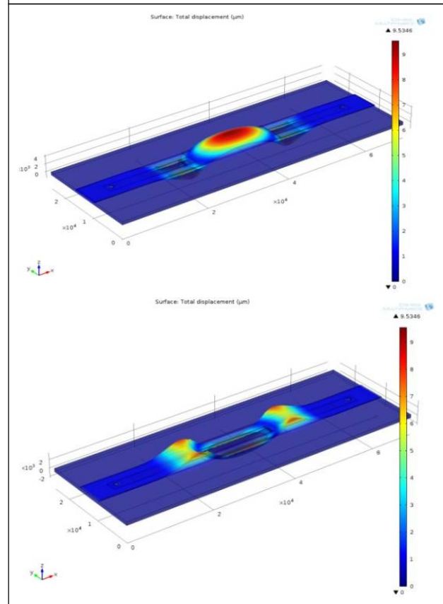
Figure 4: 3D View of Deformation of a Piezoelectric Actuator and a Membrane with a Colour Scale Representing Displacement at Current Excitation of 450 V (Top) and -450 V (Bottom)
