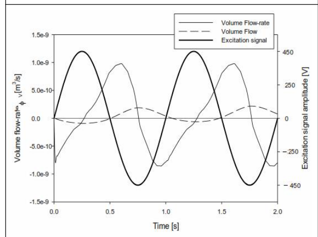
Figure 7: Time Dependent Fluid Flow at the Channel Outlet, as a Consequence of 1 Hz 450 V Sinusoidal Excitation Signal
