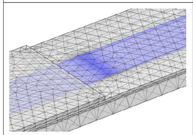
Figure 3: A Detail of Meshing at the Edge of a PMNT-PT and Around the Right Throttle
