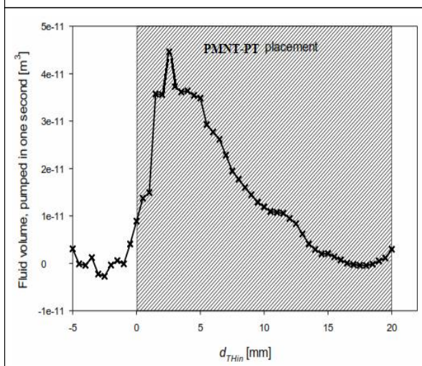
Figure 8: Fluid Volume Through the Outlet Depending on the Position of the Left Throttle Measured from the Left Edge of the PMNT-PT
