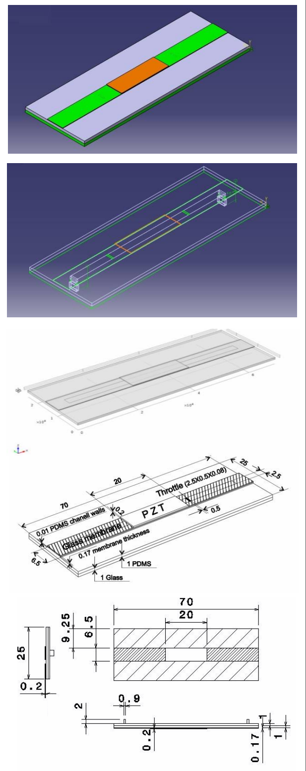
Figure 1: Top: 3D Model of a Strip Type Micro-Throttle Pump. Bottom: Dimension Details
