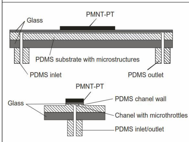
Figure 2: Cross-Section of the Proposed Structure (Dimensions are Not to Scale)
