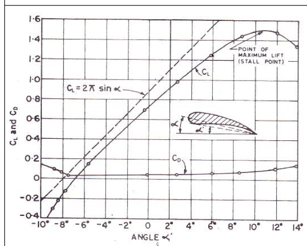
Figure 1: Angle of Attack vs. CL and CD
